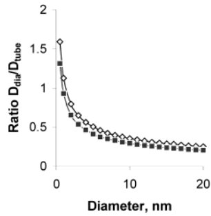
Figure 2. The ratio of the diameter of a DNR to a SWNT as a function of nanotube diameter at the conditions of equal fracture force (open diamonds) and equal weight of the structures (solid squares).
