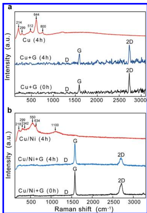
Figure 3. Raman spectrum of the Cu (a) and Cu/Ni alloy (b) foils with and without a graphene coating, acquired following heating in air at 200 °C for 0 and 4 h, respectively.
