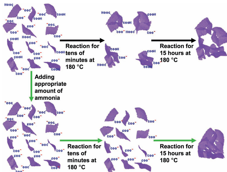
Figure 4. Process of agglomeration with the addition of different quantities of ammonia. Process of agglomeration of CGN was demonstrated by the path of black arrows. Most G-O sheets without charge were first attracted to minor G-O sheets with negative charges and became large sheets. Due to the removal of carboxyl groups, the large G-O sheets finally lost charges and agglomerated easily. Process of agglomeration of CGP was indicated by the path of green arrows. The carboxyl groups ionize into \text{COO}^- , which reduced the partial agglomeration of the initial minor G-O sheets. The G-O sheets became hydrophobic and \text{COO}^- groups were removed gradually, resulting in a uniform agglomeration of G-O sheets in a compact manner.
