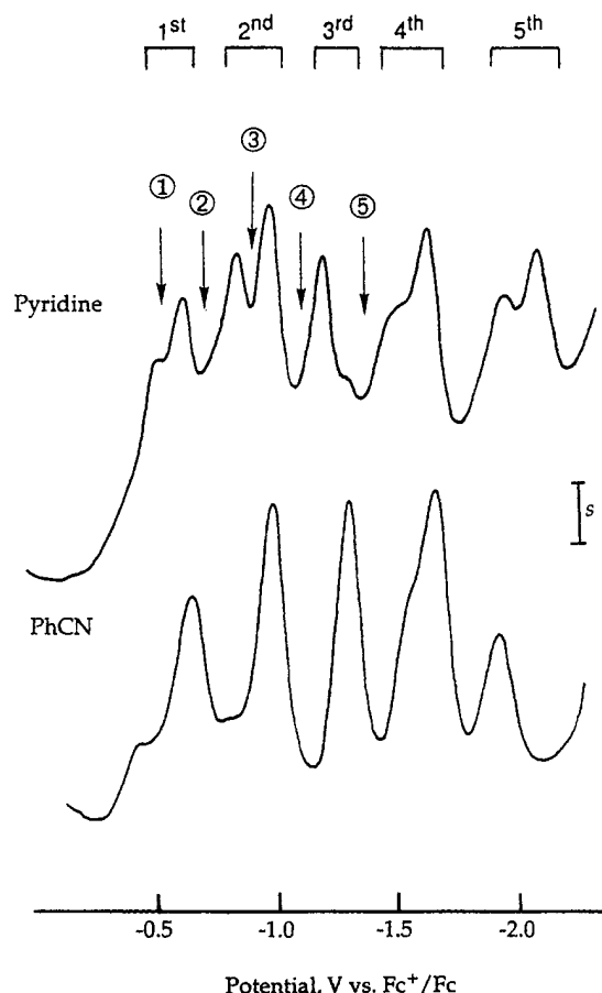
Figure 1. Differential pulse voltammograms obtained at a glassy carbon electrode for saturated solutions of C_{84} in pyridine (pulse amplitude, 40 mV; scan rate, 2 mV/s; S , 200 nA) and benzonitrile (pulse amplitude, 25 mV; scan rate, 10 mV/s; S , 100 nA). The pulse width and pulse period were kept constant and equal to 50 ms and 1 s, respectively, in both voltammograms.
