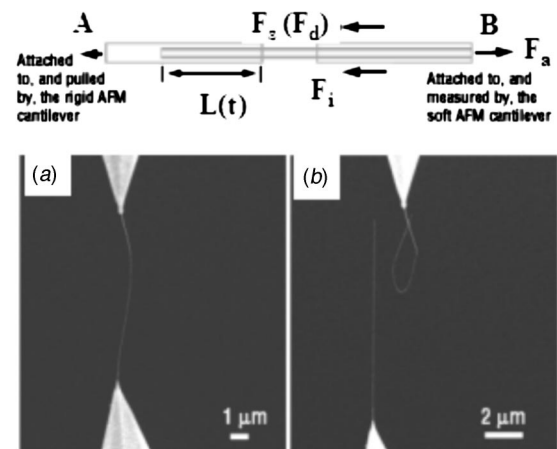
Fig. 16 The forces involved in the shell-sliding experiment can be described by F_a = F_z + F_i = \pi d \tau L(t) + F_i , where F_a is the applied pulling force as a function of time, \tau is the shear strength, L is the contact length, d the shell diameter, and F_i is a diameter dependent force originating from both surface tension and edge effects . SEM images showing the sword-in-sheath breaking mechanism of MWCNTs: (a) A MWCNT attached between AFM tips under no tensile load, (b) The same MWCNT after being tensile loaded to break. Notice the apparent overall length change of the MWCNT fragments after break compared to the initial length and the curling of the top MWCNT fragment in (b) (from [11]).
